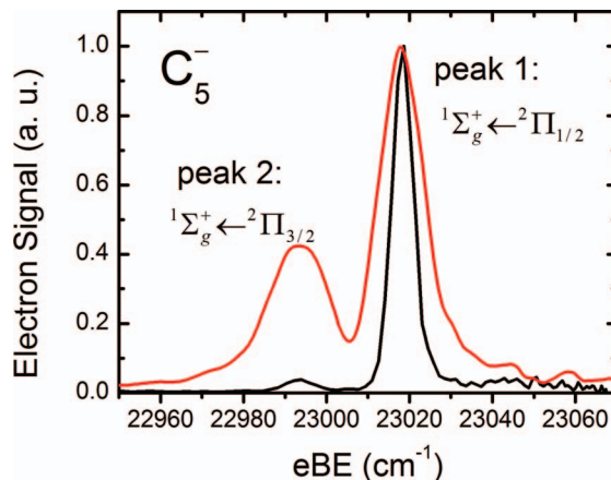
FIG. 3. Comparison of SEVI spectra of C_5^- for different experimental conditions. The spectra show the transitions from the two spin-orbit levels ^2\Pi_{1/2} (peak 1) and ^2\Pi_{3/2} (peak 2) of C_5^- to the ^1\Sigma_g^+ state of C_5 . The black curve was taken after the ion guiding and trapping system was implemented. The ion trap was held at a temperature of 5 K and the photon energy was 23\,068\text{ cm}^{-1} (black). The red curve was recorded without the ion trap at 23\,105\text{ cm}^{-1} . In this case the ions were created in a pulsed solenoid valve and directly injected into the TOFMS. All data has been transformed with the inverse-Abel method.
