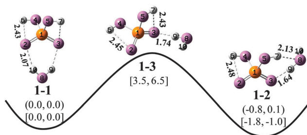
Fig. 3 Minimum energy ( 1-1 and 1-2 ) and first-order transition state ( 1-3 ) structures for the \text{H}_2\text{PO}_4^-(\text{H}_2\text{O}) complex. B3LYP/aug-cc-pVDZ and MP2/aug-cc-pVDZ relative energies (in \text{kJ mol}^{-1} ) are listed with (inside round brackets) and without (inside square brackets) ZPE corrections. The MP2 distances of hydrogen bonds are given in angstrom.
