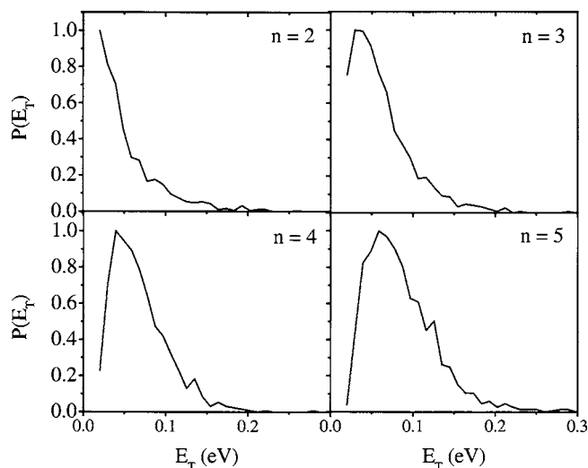
FIG. 5. Three-body P(E_T) distributions of \Gamma(\text{H}_2\text{O})_{n=2-5} excited at 3.9, 4.2, 4.4, and 4.7 eV, respectively.
