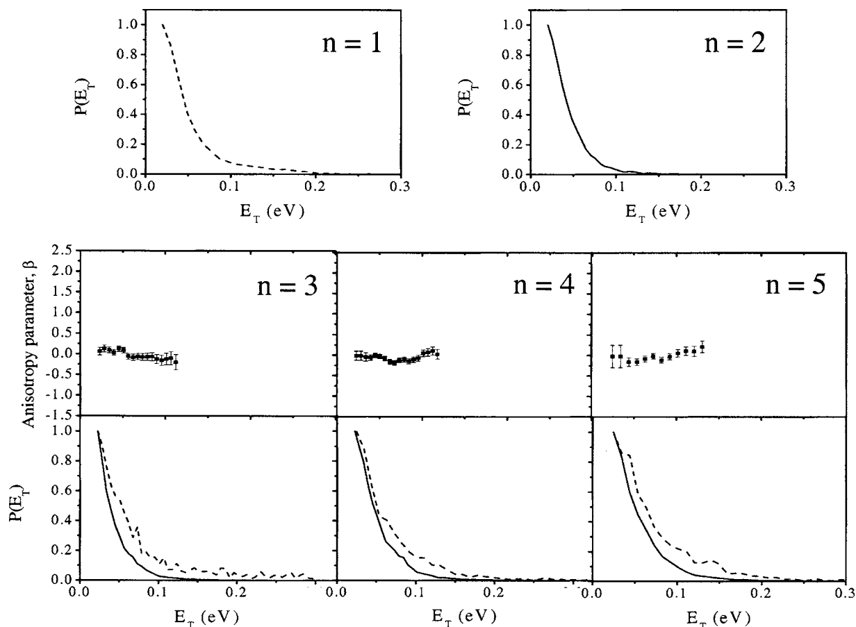
FIG. 3. Two-body translational energy distributions [ P(E_T) ] of \text{I}^-(\text{H}_2\text{O})_{n=2-5} excited at 3.9, 4.2, 4.4, and 4.7 eV, respectively (solid), as well as the P(E_T) distributions of \text{I}^-(\text{H}_2\text{O})_{n=1,3-5} excited at 5.6 eV (dashed lines). The anisotropy parameters \beta(E_T) as a function of translational energy are also shown for n=3-5 clusters excited to their CTTS states.
