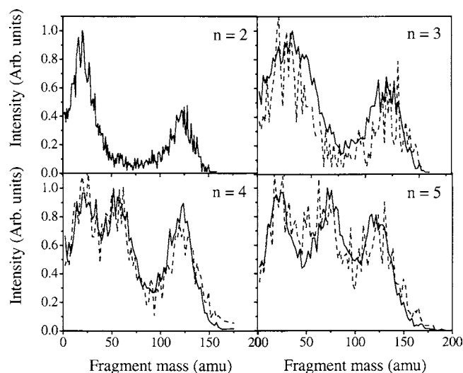
FIG. 4. Three-body photofragment mass distributions of \Gamma(\text{H}_2\text{O})_{n=2-5} excited at 3.9, 4.2, 4.4, and 4.7 eV, respectively, are shown as solid lines. The three-body photofragment mass distributions of \Gamma(\text{H}_2\text{O})_{n=3-5} excited at 5.6 eV are shown as dashed lines. The distributions correspond to the production of \text{I} (127 amu), \text{H}_2\text{O} (18 amu), and (\text{H}_2\text{O})_{n-1} [(n-1) \times 18 \text{ amu}] . The mass resolution is comparable in both cases.
