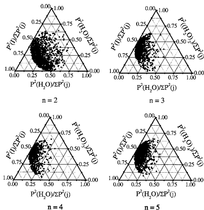
FIG. 6. Dalitz plots of \Gamma^-(\text{H}_2\text{O})_{n=2-5} excited at 3.9, 4.2, 4.4, and 4.7 eV, respectively, showing the partitioning of little momentum to the \text{H}_2\text{O} fragment and a near equal partitioning of momentum to the I and (\text{H}_2\text{O})_{n-1} fragments.
