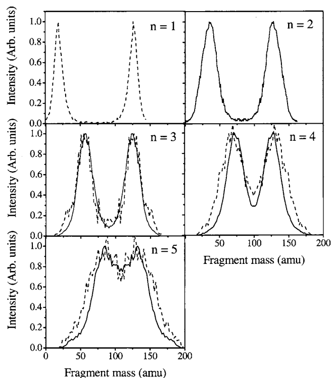
FIG. 2. Two-body photofragment mass distributions of \Gamma(\text{H}_2\text{O})_{n=2-5} excited at 3.9, 4.2, 4.4, and 4.7 eV, respectively, are shown as solid line. The two-body photofragment mass distributions of \Gamma(\text{H}_2\text{O}) excited at 4.4 eV and \Gamma(\text{H}_2\text{O})_{n=3-5} excited at 5.6 eV are shown as dashed line. The distributions correspond to the production of I (127 amu) and (\text{H}_2\text{O})_n ( n \times 18 amu).
