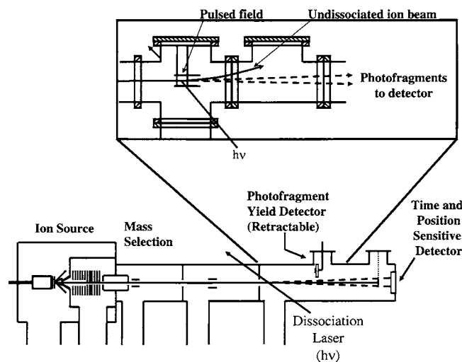
FIG. 1. Schematic of the fast beam coincidence imaging apparatus. Detail of the interaction region showing the pulsed field used to deflect undissociated parent ions from striking the detector is also shown.
