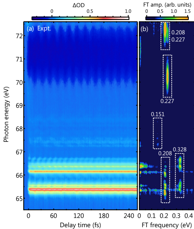
FIG. 2. (a) Experimental delay-dependent transient-absorption spectra of DBr. The pump and probe pulses are parallelpolarized. Multiple quantum beats are resolved, showing the electronic and vibrational coherences induced by the strong-field ionization. (b) Fourier transformation (FT) of the experimental spectra along the delay axis. Main FT components are marked by dashed boxes with the numbers indicating the beat frequencies in units of eV.
