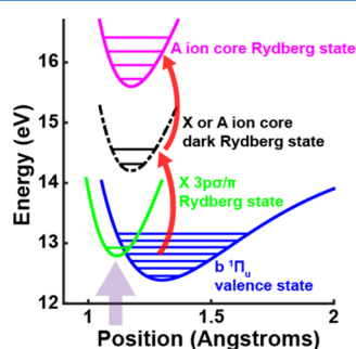
Figure 7. Schema showing the origin of the subcycle oscillations. A dark state built on the A\ ^2\Pi_u N_2^+ core is shown to illustrate the Franck–Condon overlap with the b\ ^1\Pi_u vibrational levels. The red arrows symbolize NIR-induced population transfer. The purple arrow indicates the Franck–Condon overlap with the ground state of nitrogen.
