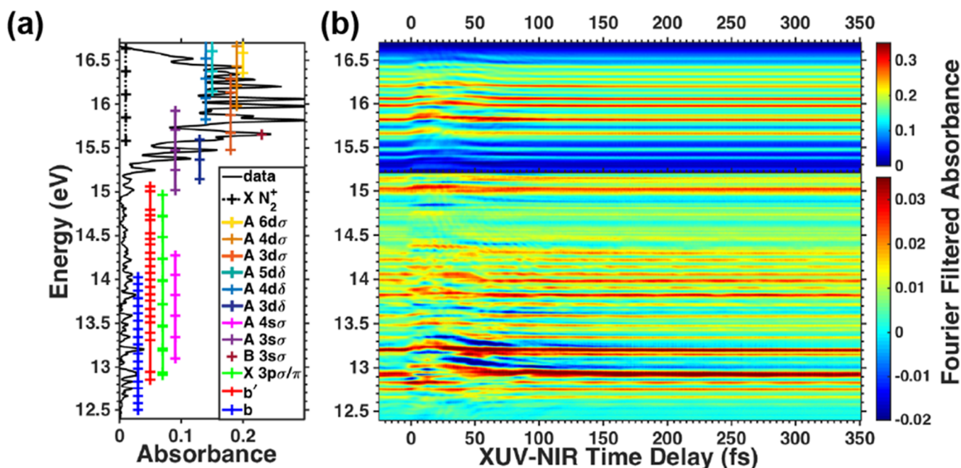
Figure 3. (a) Static absorption of nitrogen. Positions of vibrational levels of the valence b\ ^1\Pi_u (blue) and b'\ ^1\Sigma_u^+ (red) states and of the Rydberg series built on the X\ ^2\Sigma_g^+ N_2^+ (green) and A\ ^2\Pi_u N_2^+ cores are indicated. 31,34,40,47–49 (b) Nitrogen transient absorption measurement in the 12.5 to 16.7 eV photon energy range. The color scale represents absorbance that has been Fourier filtered. The NIR pulse arrives after the XUV pulse for positive time delays.
